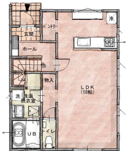
1F
